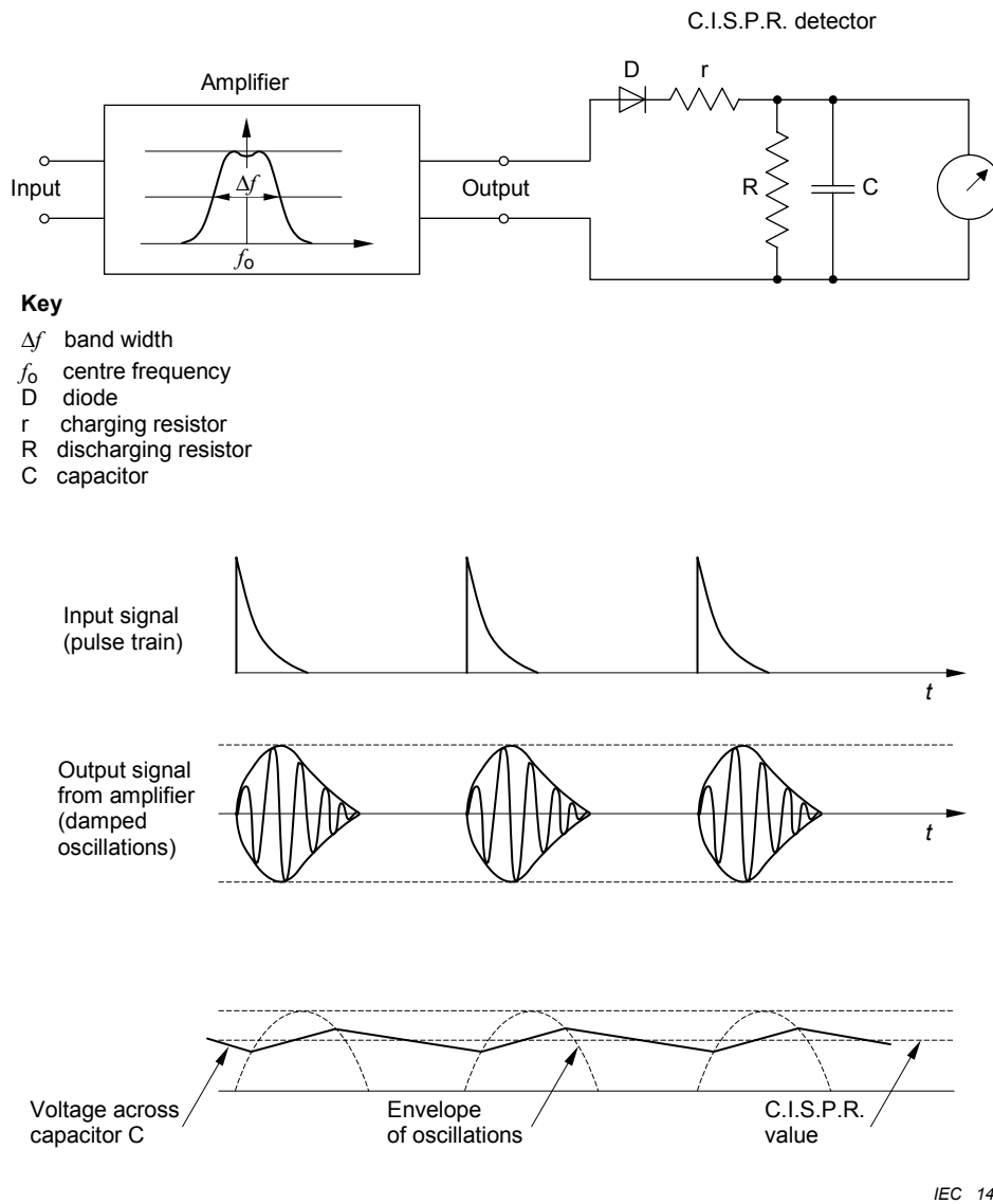
Figure 1 – Transformation of pulses through a CISPR measuring receiver
