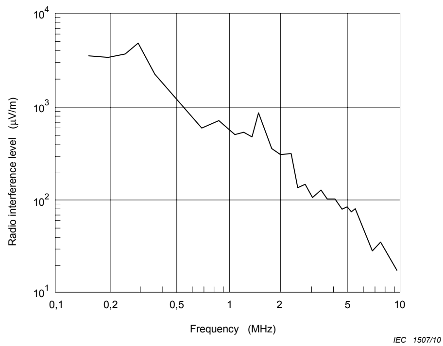
Figure 18 – Example of frequency spectrum of the radio interference in the vicinity of a d.c. line (30 m) at a short distance from the converter station
