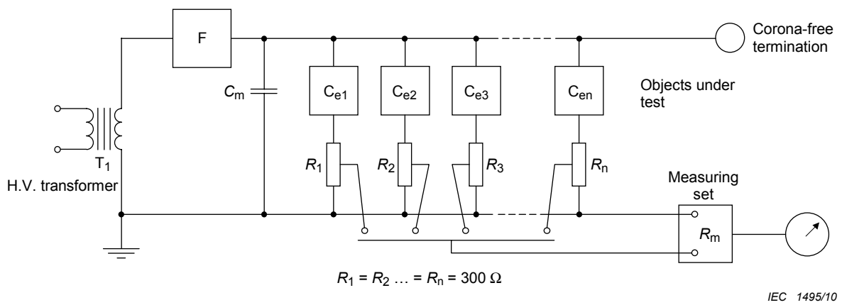
Figure 8 – Special test circuit
