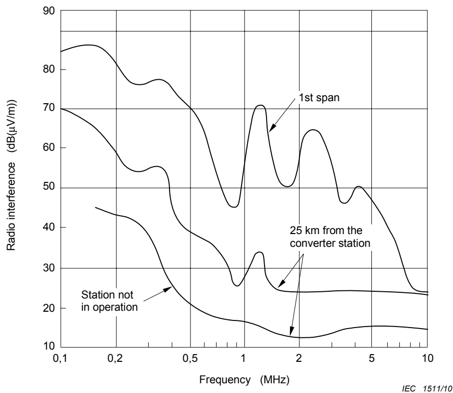
Figure 22 – Frequency spectra of the radio interference recorded along a 200 kV d.c. line, at 20 m from the conductor, at different distances from the converter station
